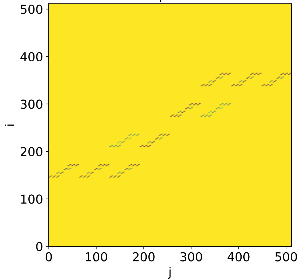
heatmap of cost matrix c_{ij} with n = 8
