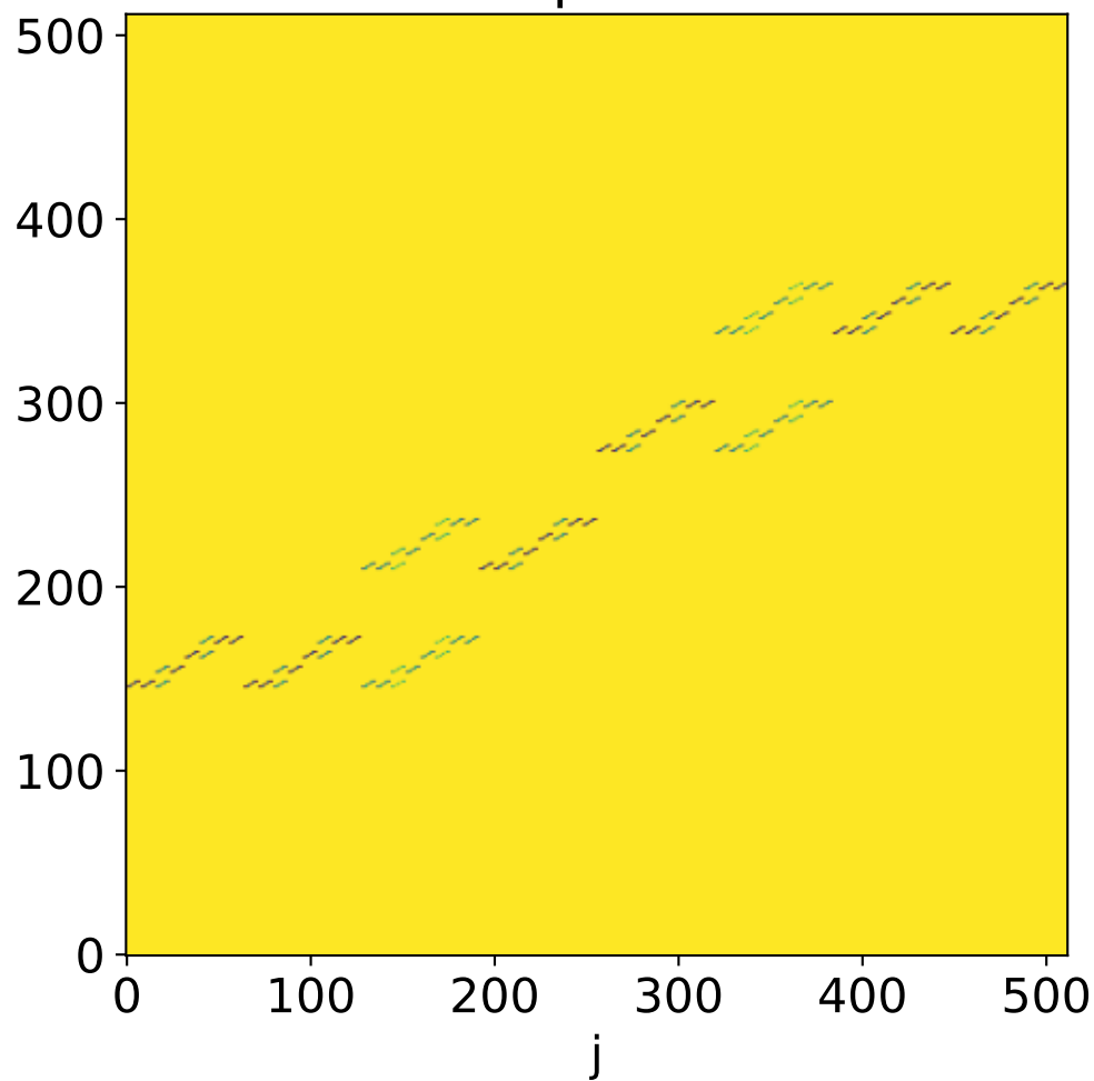
heatmap of cost matrix c_{ij} with n = 8
